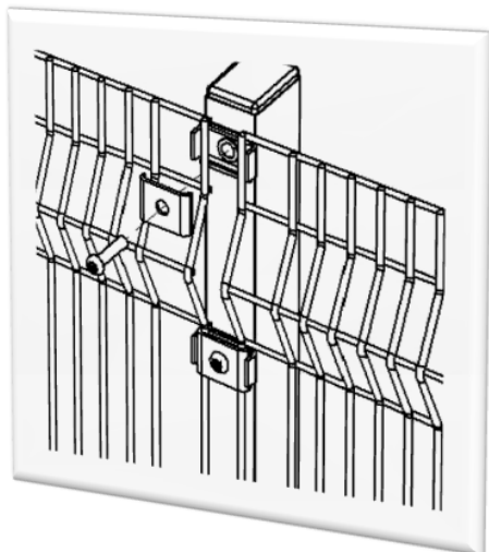
Standard Post & Panel Fixing
